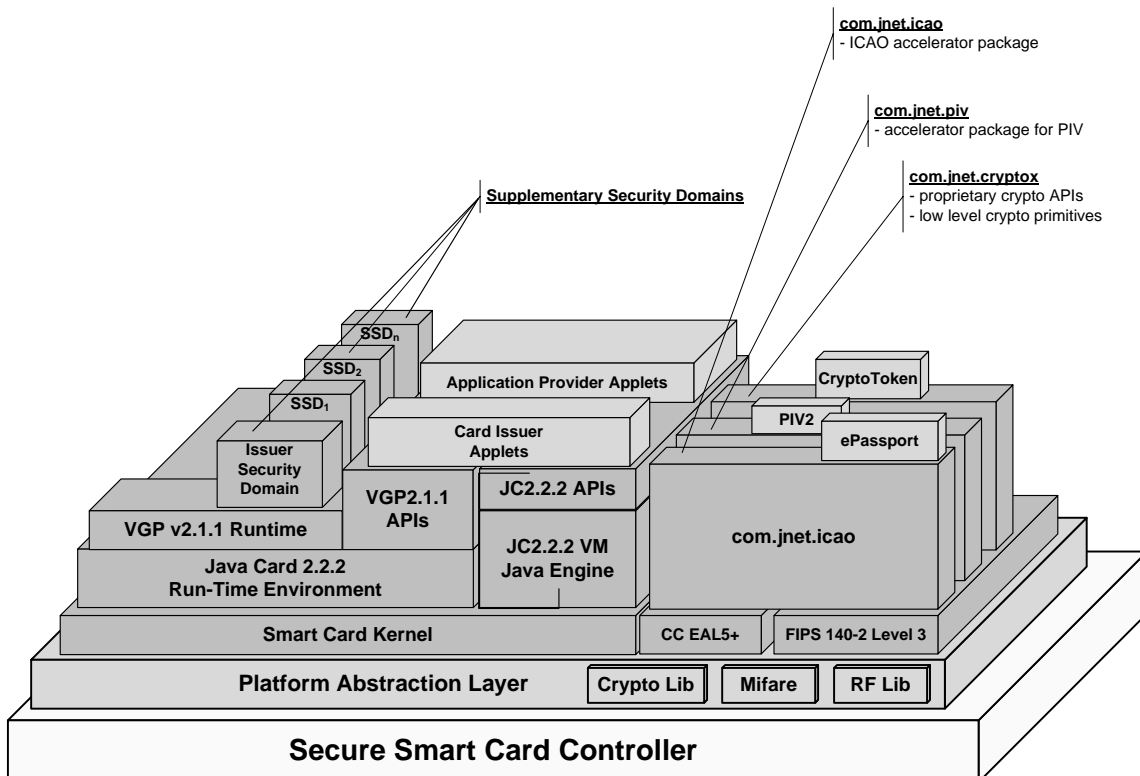
Figure 1. Internal representation of jNet’s JC222/VGP2.1.1 offering.
